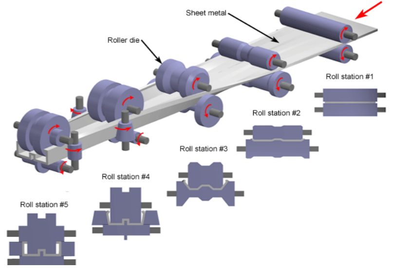
Schematic
