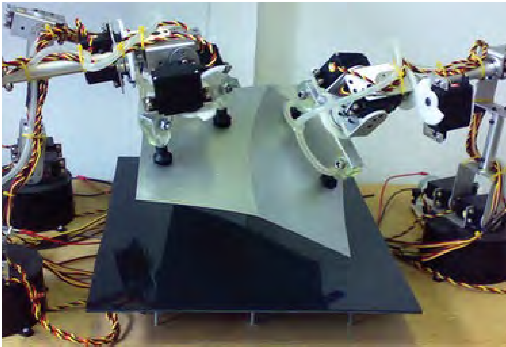
Robot folding a metal sheet
