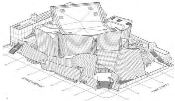
Construction Frame
